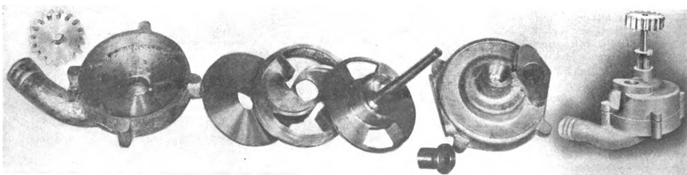
Fig. 6.—Detailed parts and complete assembly of a form of centrifugal pump.
